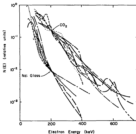
Fig. 54. Composite of spectra taken with both the Nd:glass (Intensity, \sim 5 \times 10^{15} W/cm 2 ) and CO 2 (Intensity \sim 3 \times 10^{14} W/cm 2 ) lasers. 2 Seven spectra taken with the Nd:glass laser and nine spectra from the CO 2 laser are normalized to their average value, at 200-keV energy. In both cases the standard deviation of the ratios of normalization constants was \sim 4 . The relative intensity between the averages for the two lasers is preserved.
