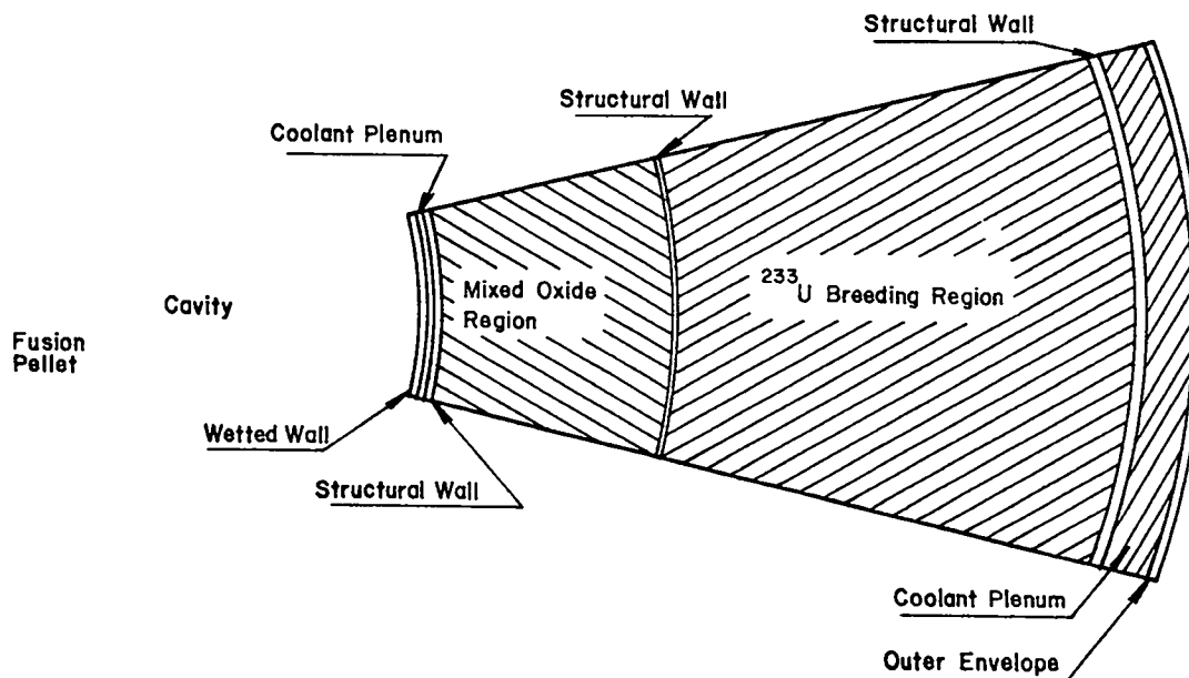
Fig. 88. Conceptual design of 239 Pu-burner/ 233 U-breeder hybrid reactor.
