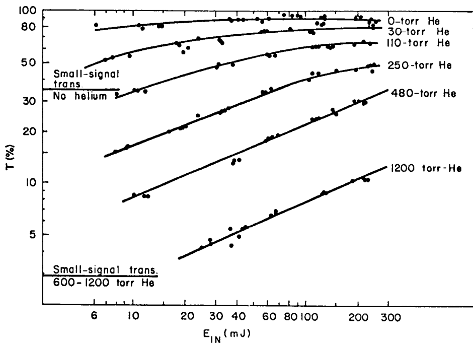
Fig. 30. Observed energy transmissivity of 10-torr C_2H_4 with various partial pressures of helium at 10.59 \mu m in a cell 122 cm long.
